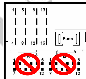
MOST connector at head unit
